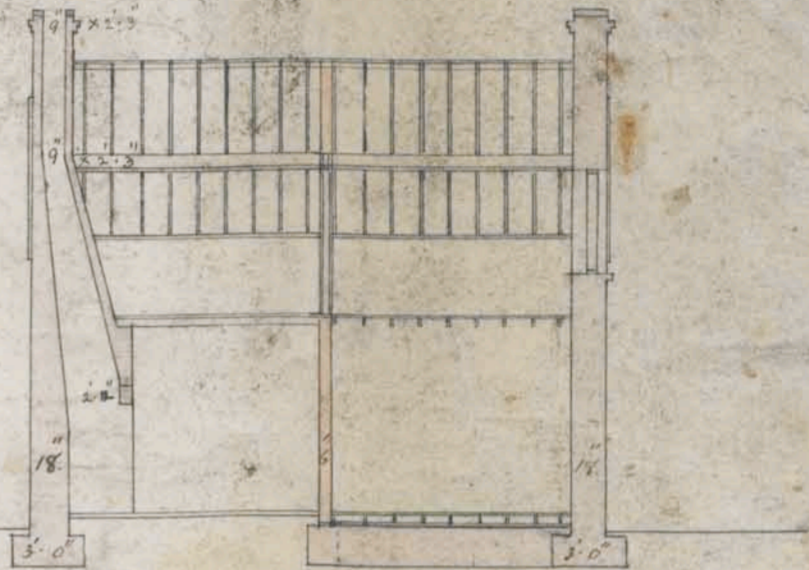
SECTION THRU C.D.
